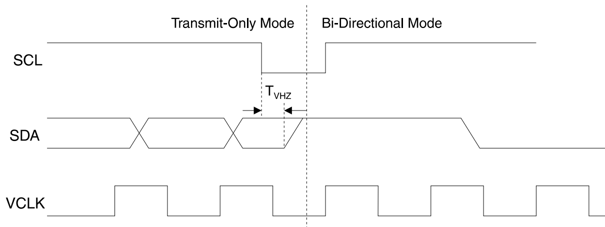
Figure 3. Mode Transition
