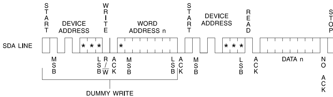
Figure 8. Random Read
