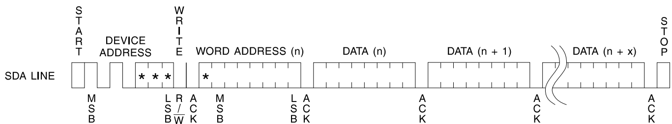
Figure 6. Page Write
