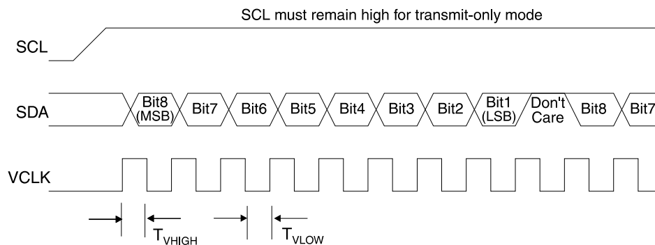
Figure 1. Transmit-Only Mode
