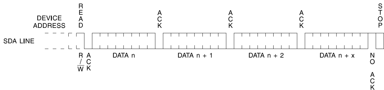
Figure 9. Sequential Read
