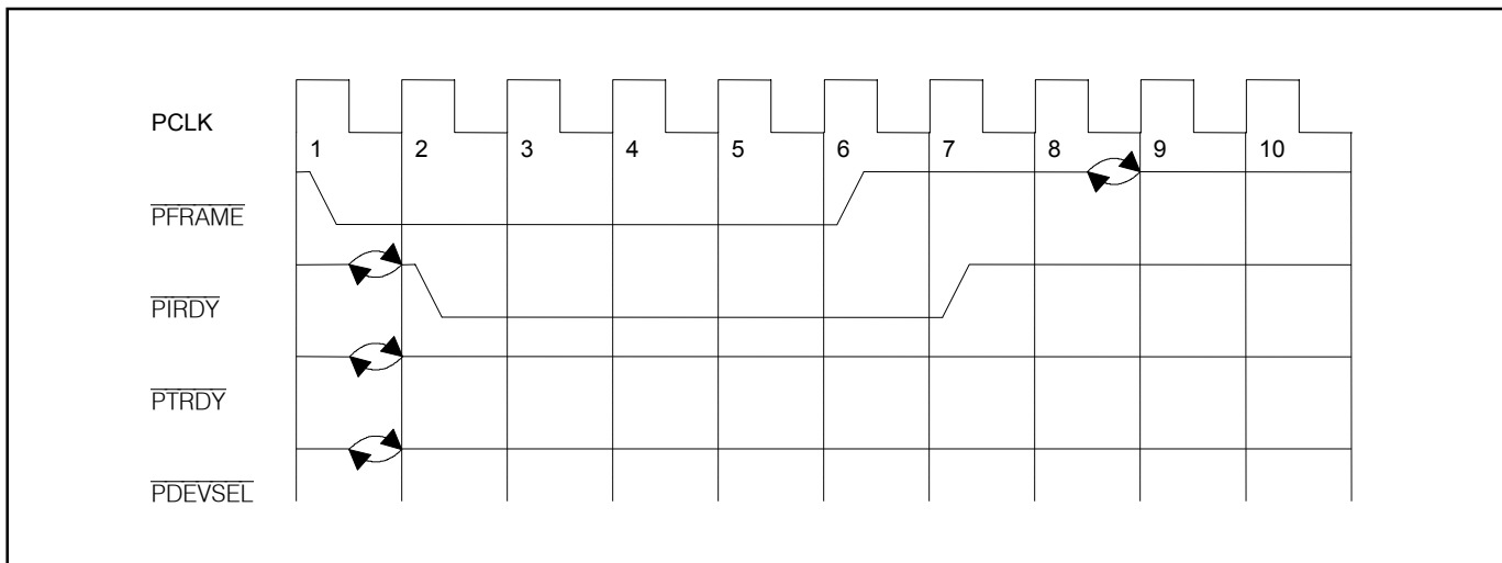
Figure 10-5. PCI Initiator Abort
