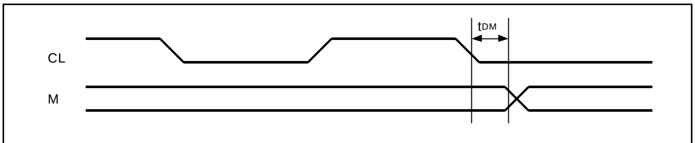
Figure 38. Display Control Output Timing
