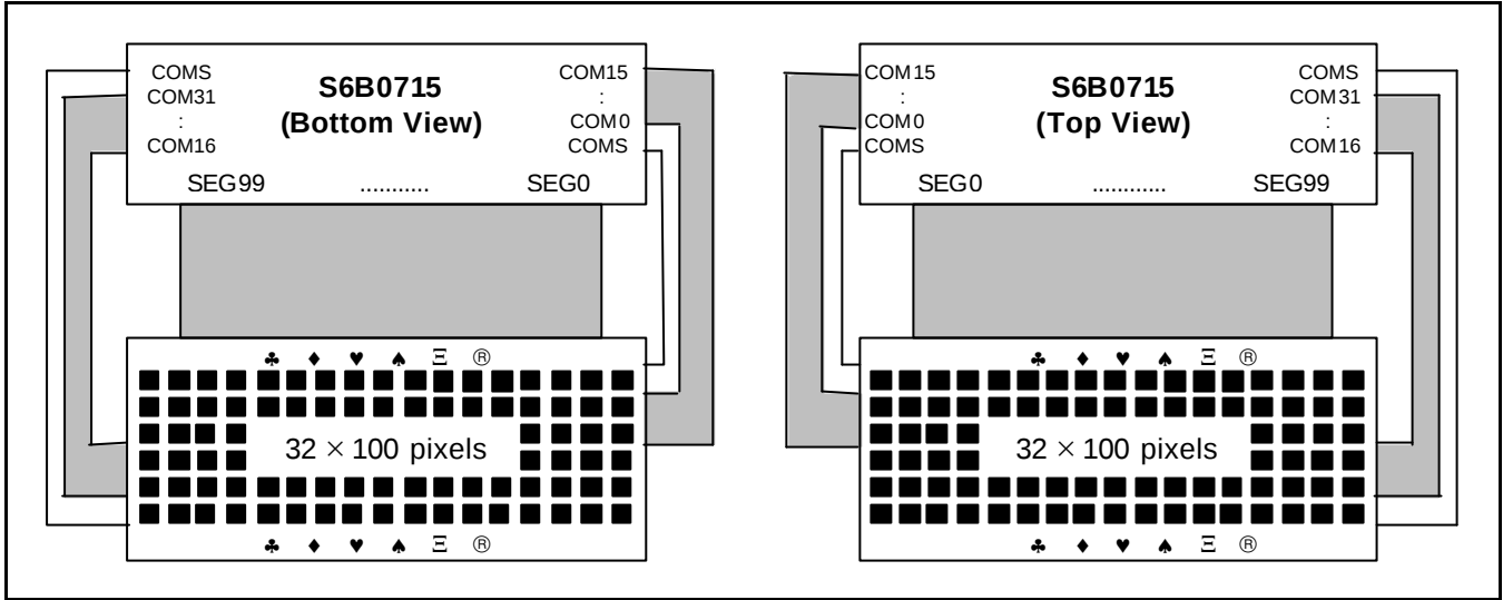
Figure 42. SHL = 0, ADC = 1
