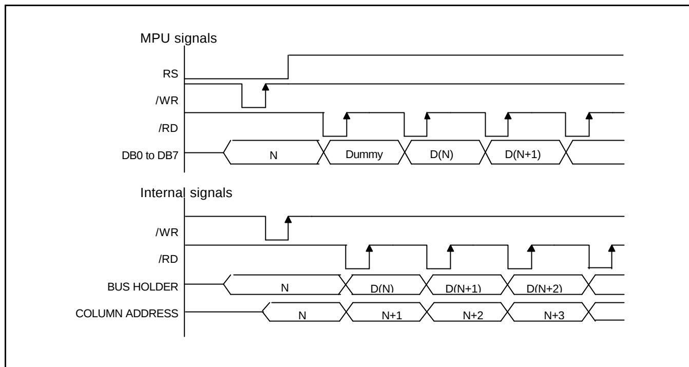
Figure 7. Read Timing
