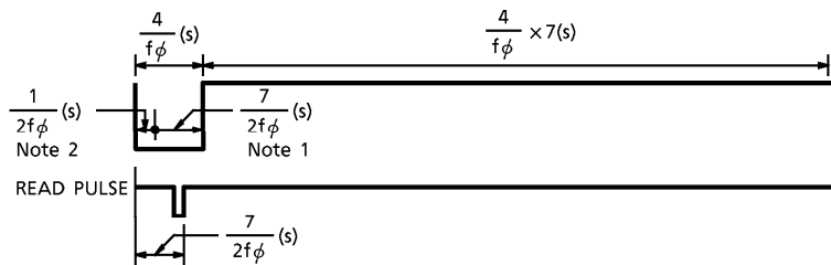
(Note 1, 2, 5) RESET Waveform, 1-cycle
