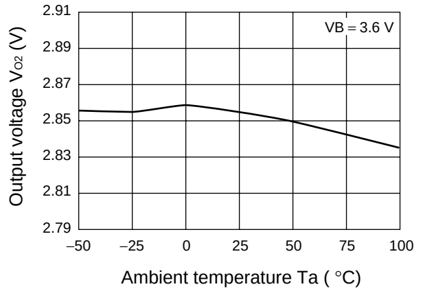
Output voltage vs. ambient temperature (BBREG2)
