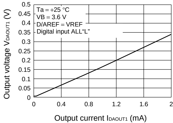
DA1 output voltage vs. output current
