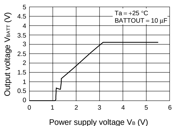
Output voltage vs. power supply voltage (BATTREG)
