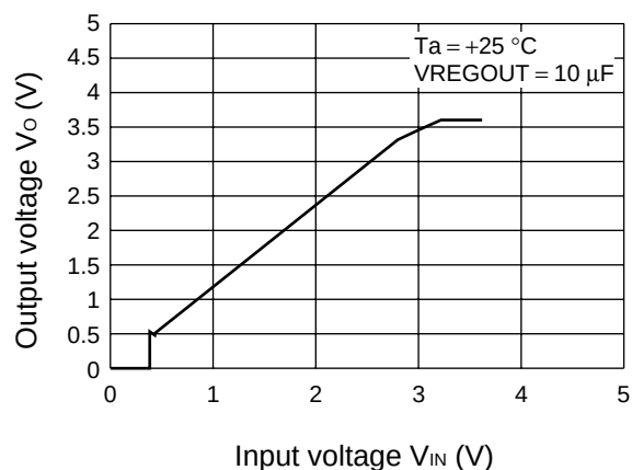
Output voltage vs. input voltage (Variable REG)
