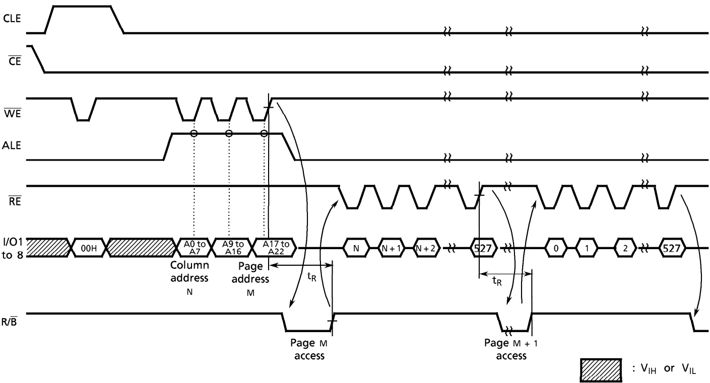
Sequential Read (1) Timing Diagram
