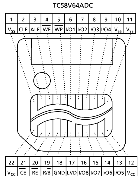
Figure 1. Pinout
