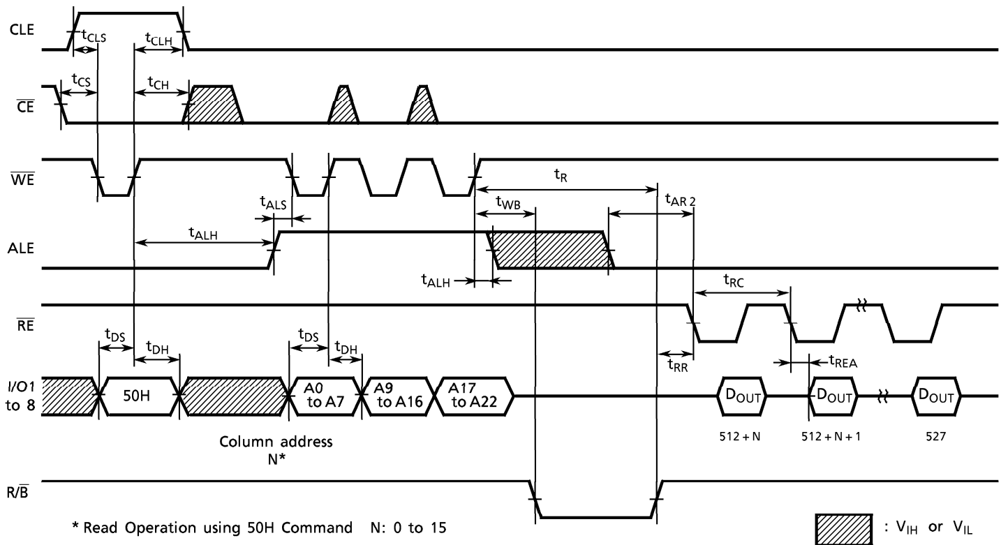
Read Cycle (3) Timing Diagram
