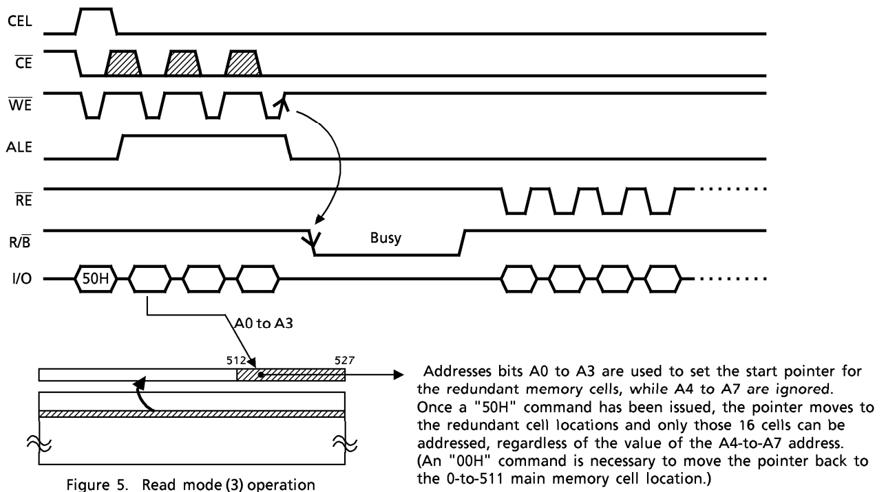
Figure 5. Read mode (3) operation
