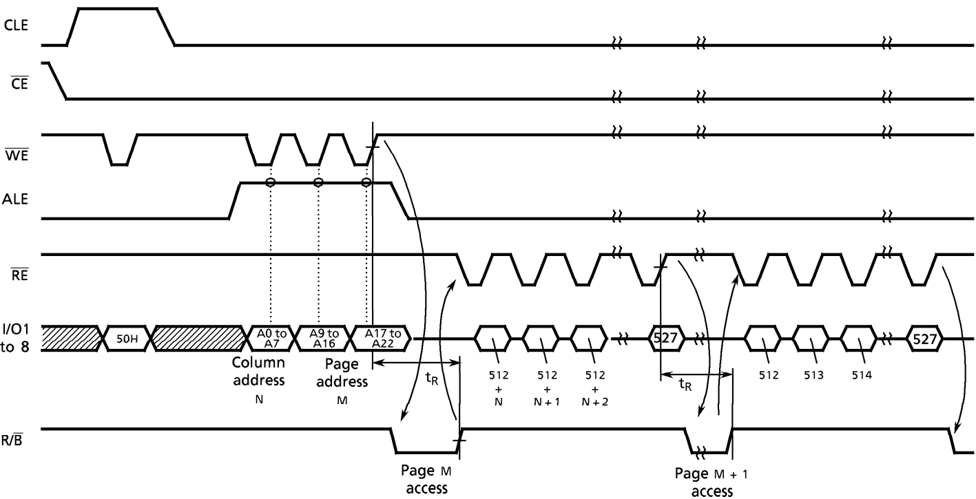
Sequential Read (3) Timing Diagram
