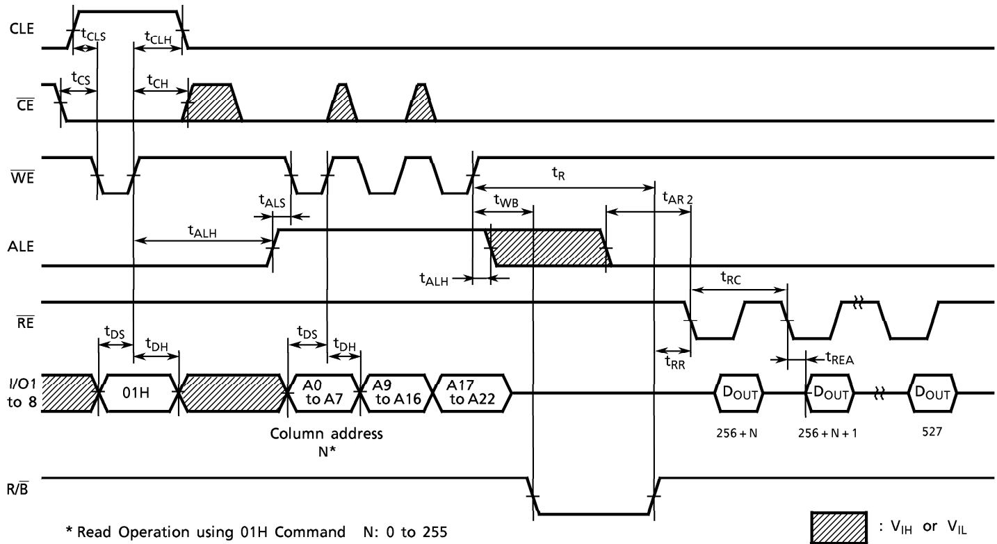
Read Cycle (2) Timing Diagram
