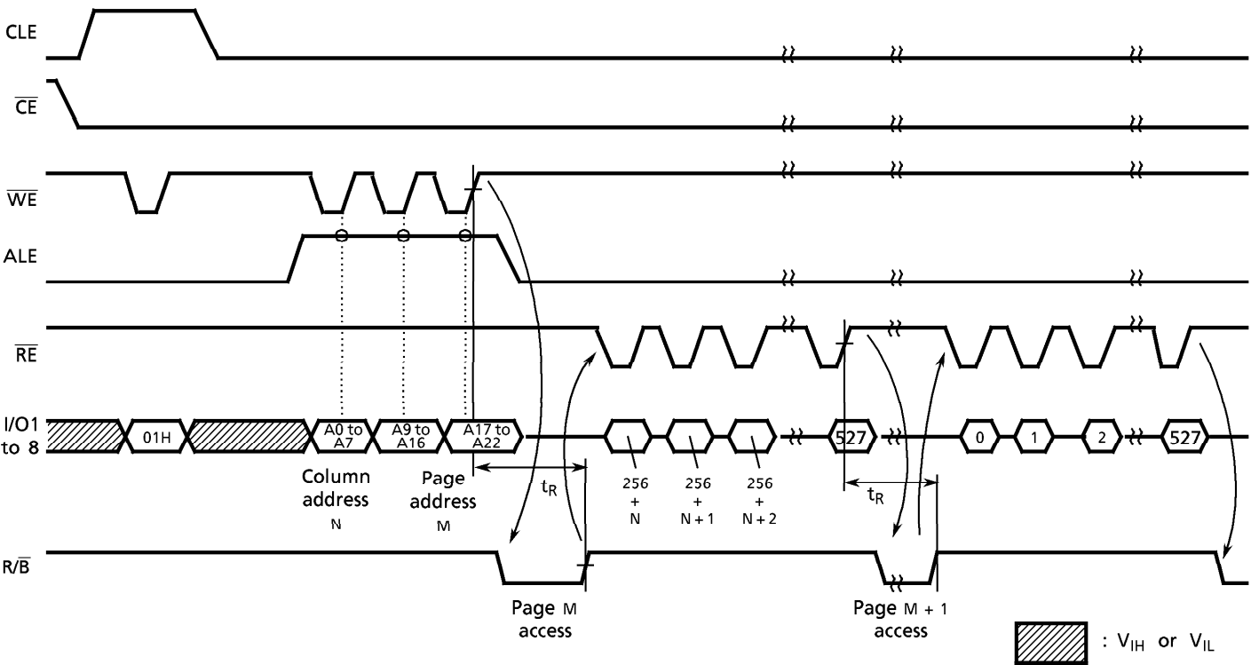
Sequential Read (2) Timing Diagram
