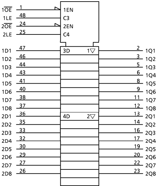
IEC LOGIC SYMBOL
