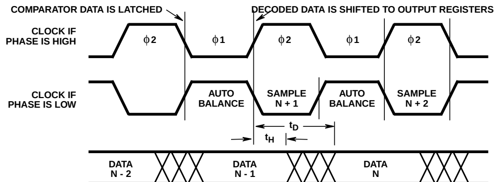
FIGURE 1. INPUT-TO-OUTPUT
