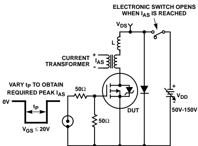
FIGURE 21. UNCLAMPED ENERGY TEST CIRCUIT
