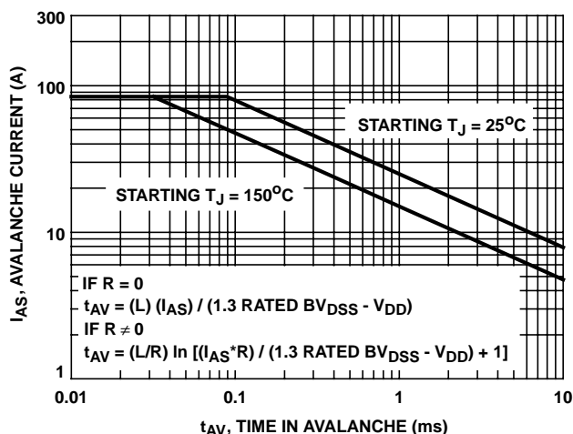
FIGURE 20. UNCLAMPED INDUCTIVE SWITCHING
