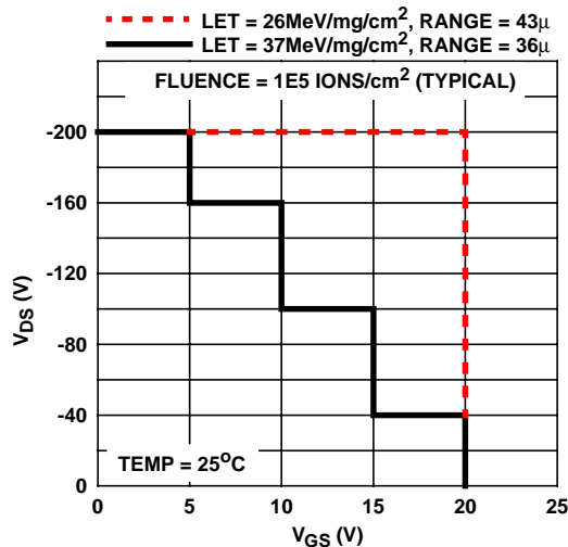
FIGURE 13. SINGLE EVENT EFFECTS SAFE OPERATING AREA
