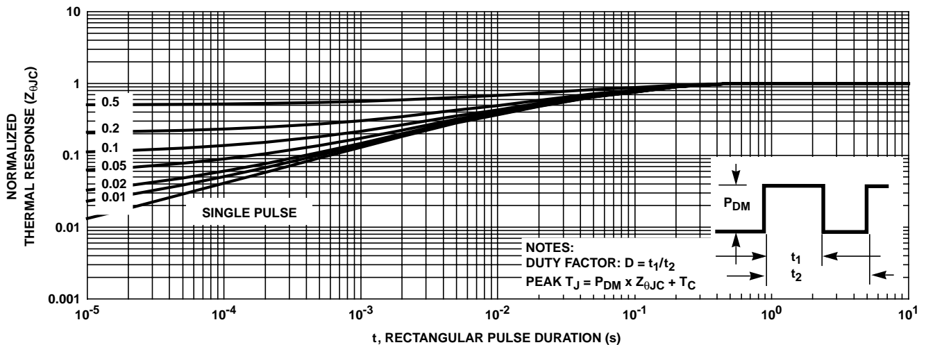
FIGURE 19. NORMALIZED MAXIMUM TRANSIENT THERMAL RESPONSE
