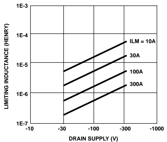
FIGURE 14. DRAIN INDUCTANCE REQUIRED TO LIMIT GAMMA DOT CURRENT TO I_{AS}
