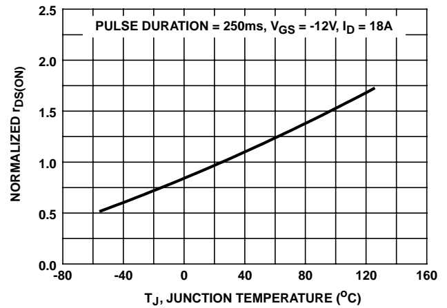
FIGURE 18. NORMALIZED r_{DS(ON)} vs JUNCTION TEMPERATURE
