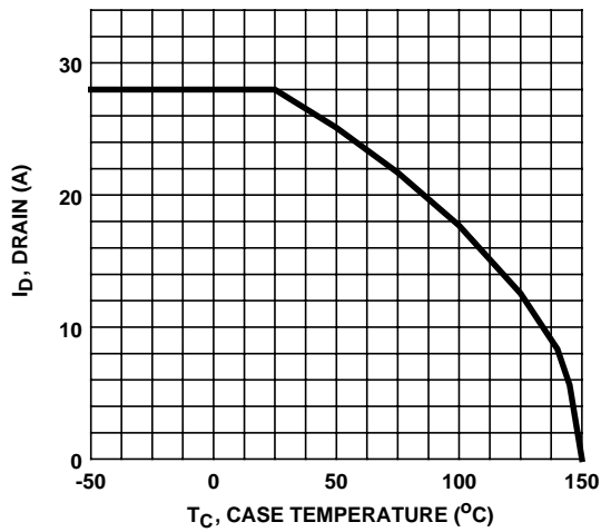
FIGURE 15. MAXIMUM CONTINUOUS DRAIN CURRENT vs TEMPERATURE
