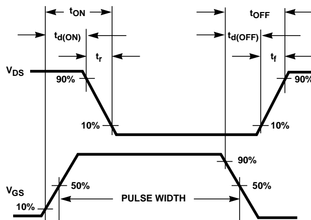
FIGURE 24. RESISTIVE SWITCHING WAVEFORMS
