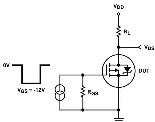
FIGURE 23. RESISTIVE SWITCHING TEST CIRCUIT
