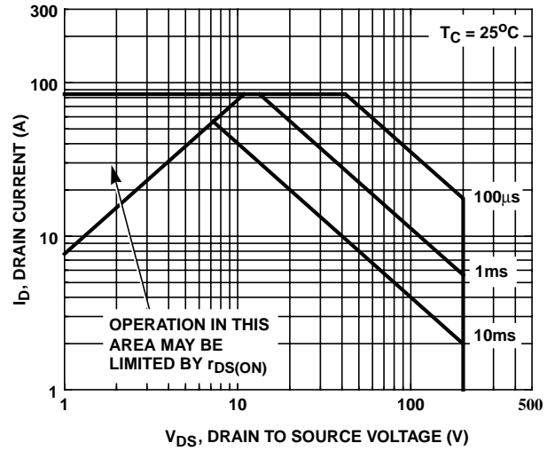
FIGURE 16. FORWARD BIAS SAFE OPERATING AREA
