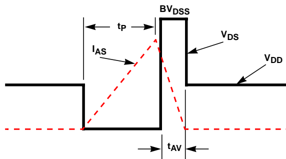
FIGURE 22. UNCLAMPED ENERGY WAVEFORMS
