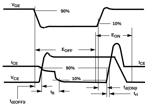
FIGURE 21. SWITCHING TEST WAVEFORMS
