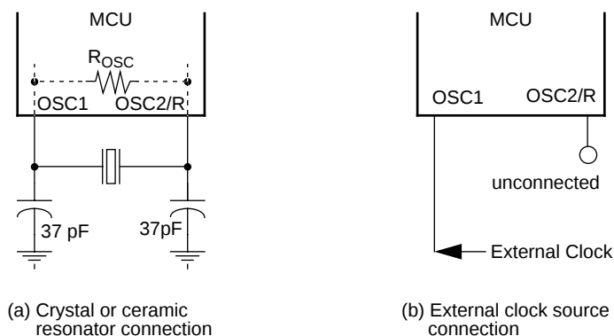
Figure 1-3. Oscillator Connections
