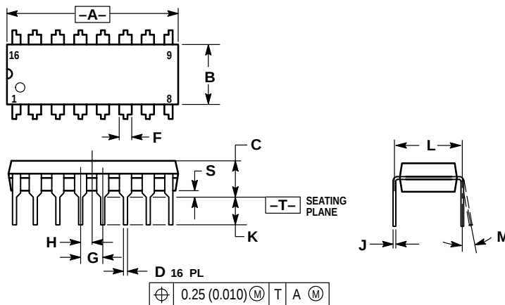
Figure 12-1. 16-Pin PDIP Mechanical Dimensions
