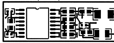
Maximum Components placed on one side
