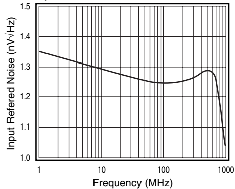
Input Noise
