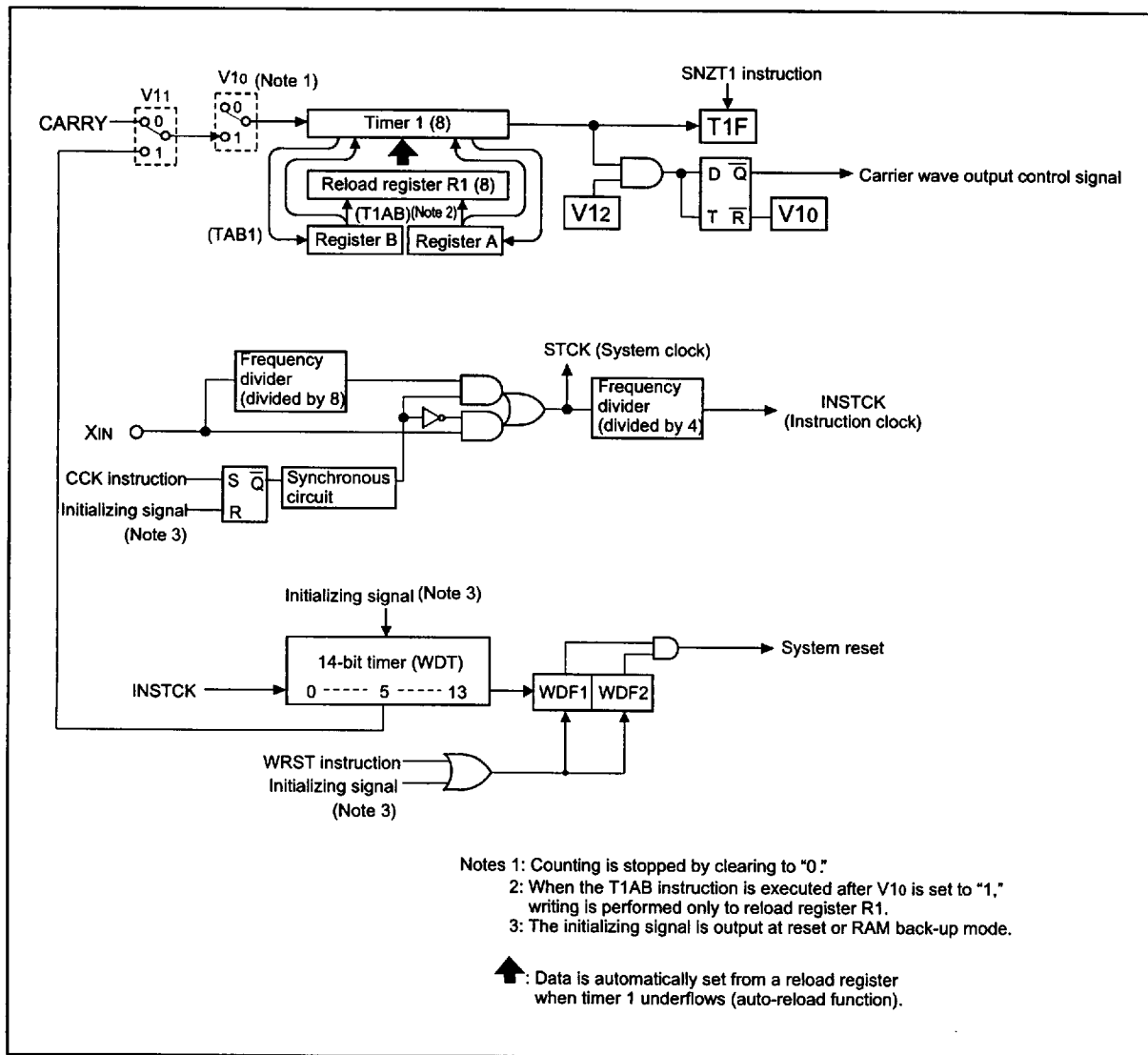
Fig. 13 Timers structure
