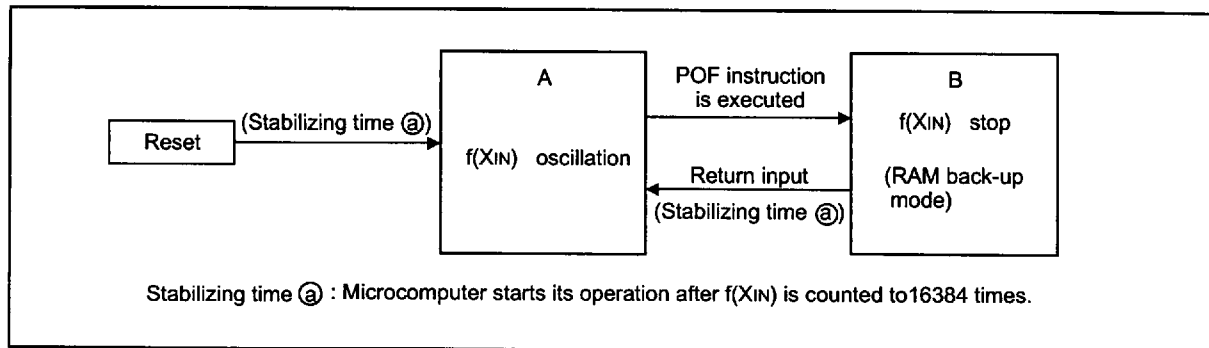
Fig. 21 State transition
