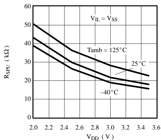
Figure 72. Strong pull-up resistor vs. V_{DD}
