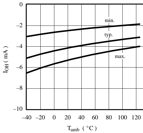
Figure 78. Output high current vs. T_{amb} = 25^{\circ}C V_{DD} = 3.0 V, V_{OH} = 0.8 \times V_{DD}
