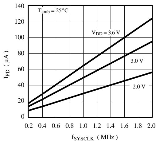
Figure 60. Power-down supply current vs. frequency
