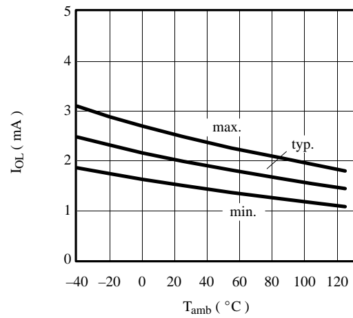
Figure 79. Output low current vs. T_{amb} V_{DD} = 2.0 V, V_{OL} = 0.2 \times V_{DD}
