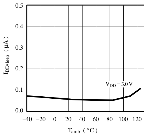
Figure 61. Sleep current vs. T_amb
