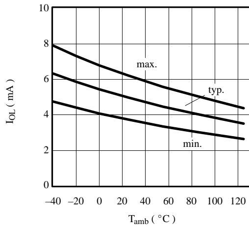
Figure 77. Output low current vs. T_{amb} V_{DD} = 3.0 V, V_{OL} = 0.2 \times V_{DD}
