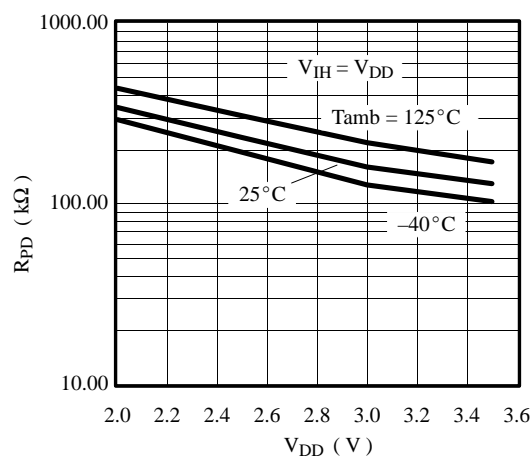
Figure 74. Pull-down resistor vs. V_{DD}
