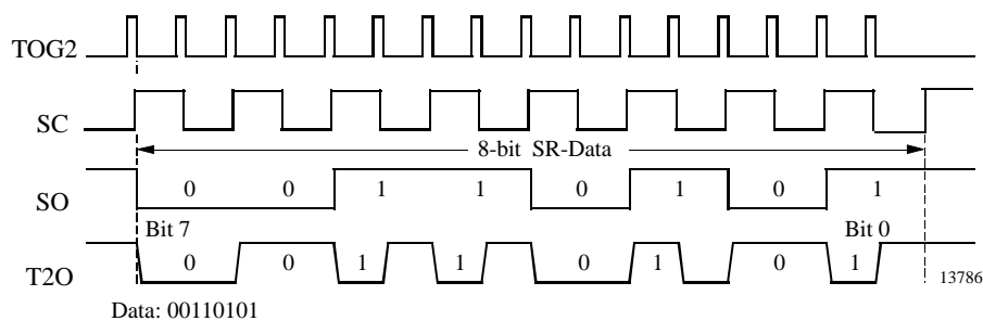
Figure 39. Biphasic modulation
