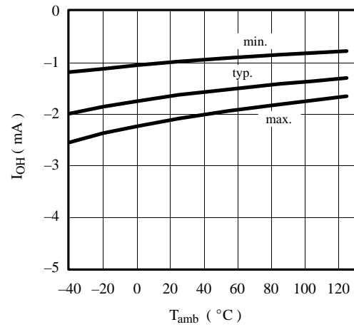
Figure 80. Output high current vs. T_{amb} = 25^{\circ}C V_{DD} = 2.0 V, V_{OH} = 0.8 \times V_{DD}
