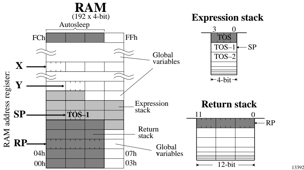
Figure 5. RAM map
