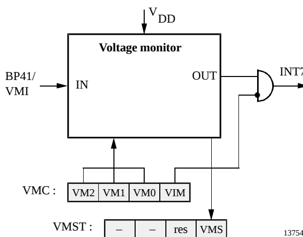
Figure 11. Voltage monitor
