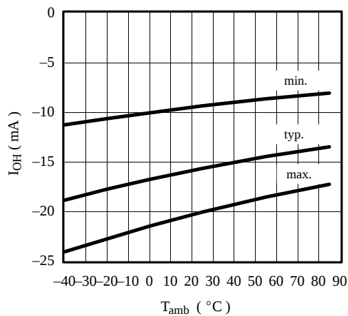
Figure 108. Output high current vs. V_{DD} = 6.5\text{ V} , V_{OH} = 0.8 \times V_{DD}
