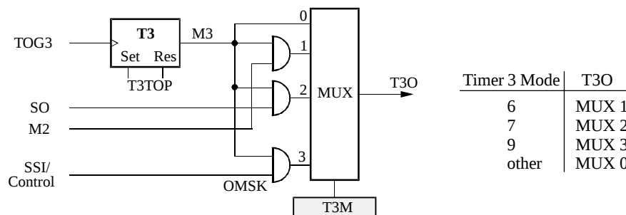
Figure 56. Modulator 3
