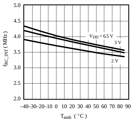
Figure 99. Internal RC frequency vs. T_{amb}
