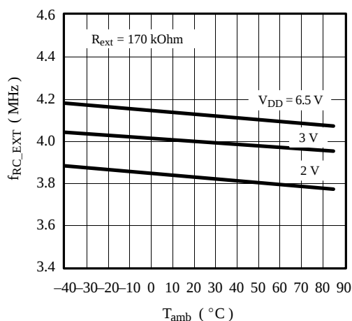
Figure 100. External RC frequency vs. T_{amb}
