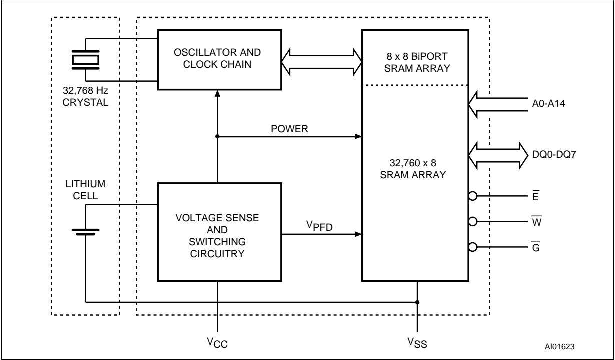
Figure 6. Block Diagram
