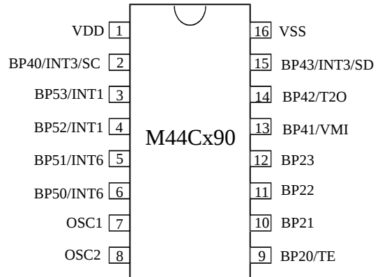
Figure 4. Pin connections for M44Cx90 in SO16 package
