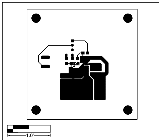
Figure 3. MAX1797 EV Kit PC Board Layout—Component Side
