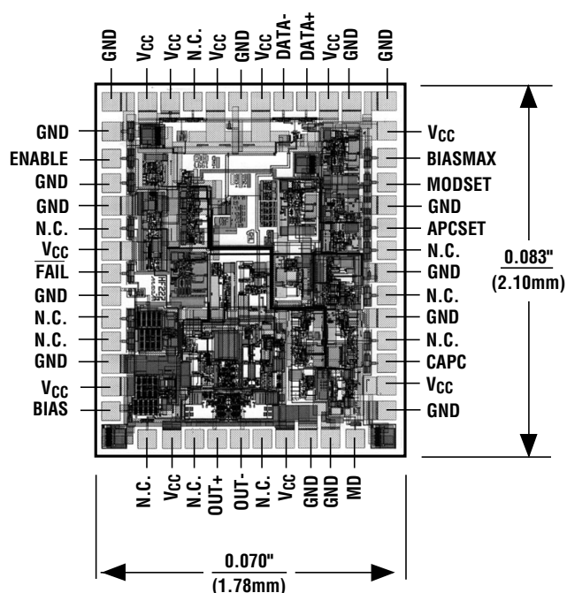
Chip Topography
