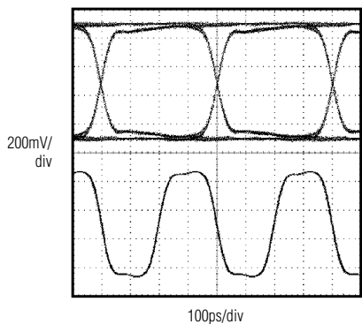
RECOVERED CLOCK AND DATA (2.488Gbps, 2^{23} - 1 PATTERN, V_{IN} = 10mV_{P-P} )
