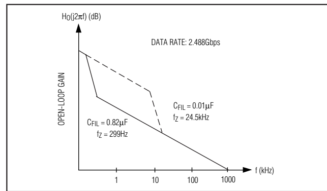
Figure 6. Open-Loop Transfer Function
