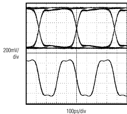
RECOVERED CLOCK AND DATA (2.67Gbps, 2^{23} - 1 PATTERN, V_{IN} = 10mV_{P-P} )
