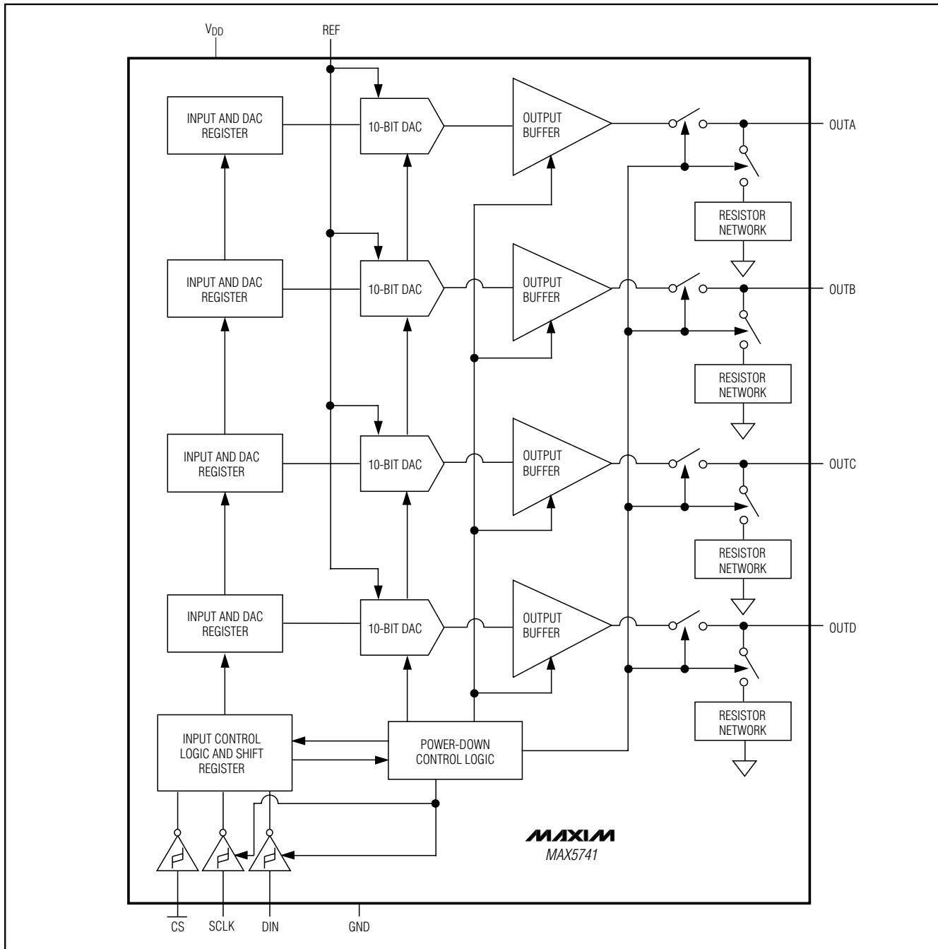
Functional Diagram
