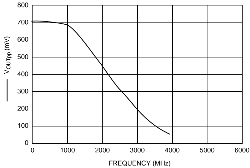
Figure 4. F_{max} Typical
