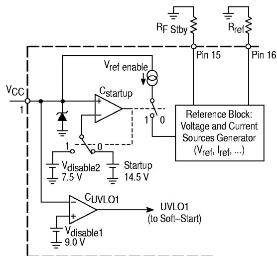
Figure 47. V_{CC} Management
