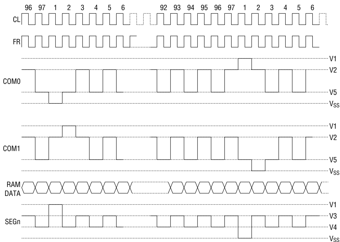
Fig. 5(b) Waveforms in the line reversal drive method
