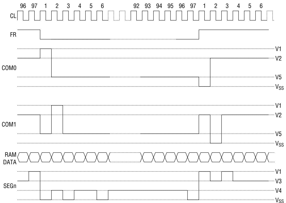
Fig. 5(a) Waveforms in the frame reversal drive method
