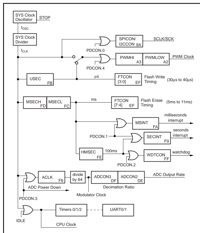
FIGURE 4. MSC1211 Timing Chain and Clock Control.
