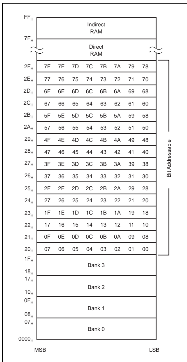
FIGURE 13. Scratchpad Register Addressing.
