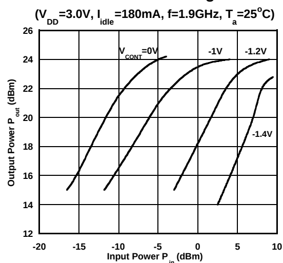
Output Power vs. Input Power vs. Control Voltage
