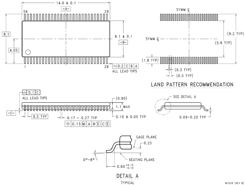
56-Lead Molded Thin Shrink Small Outline Package, JEDEC Order Number DS90CF581MTD NS Package Number MTD56
