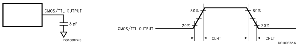
FIGURE 3. DS90CR288 (Receiver) CMOS/TTL Output Load and Transition Times
