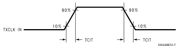
FIGURE 4. DS90CR287 (Transmitter) Input Clock Transition Time
