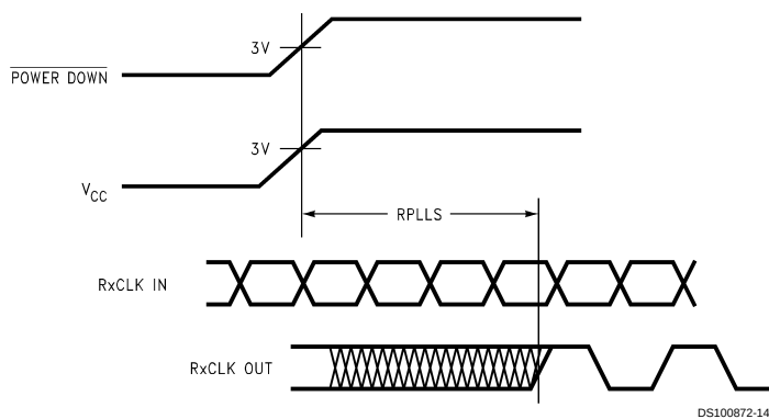
FIGURE 11. DS90CR288 (Receiver) Phase Lock Loop Set Time
