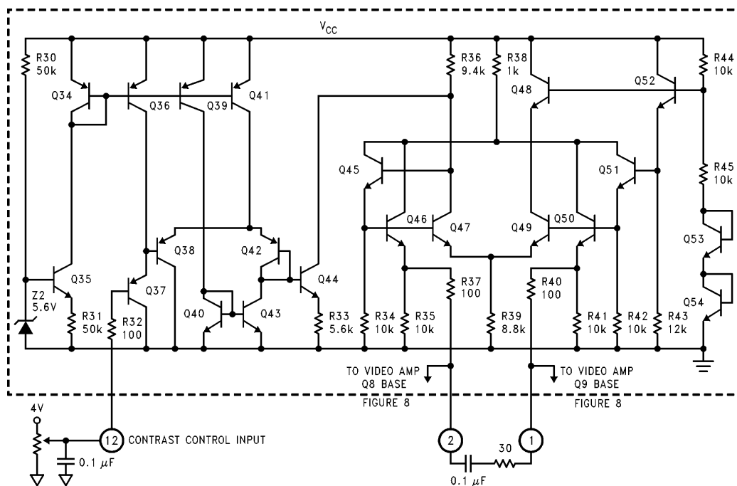
FIGURE 9. Simplified Schematic of LM1205 Contrast Control
