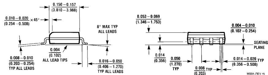
SO Package (M) Order Number LM334M or LM334SM NS Package Number M08A
