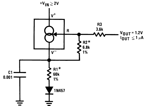
1.2V Reference Operates on 10 \mu\text{A} and 2V
