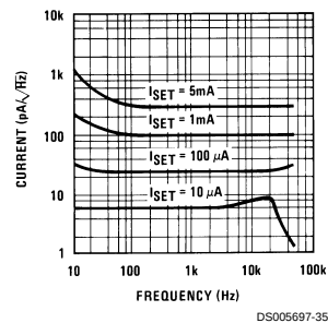
Current Noise
