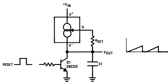
Ramp Generator
