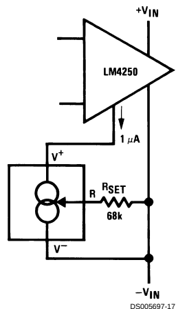
Micropower Bias
