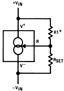
Generating Negative Output Impedance
