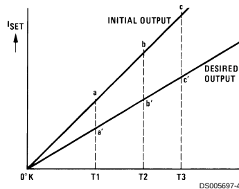
FIGURE 2. Gain Adjustment
