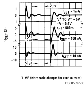
Transient Response
