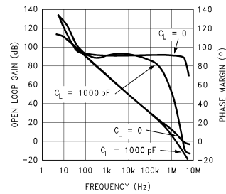
Gain and Phase, 2.7V Supply
