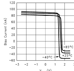
Inverting Input, Bias Current vs Common Mode Voltage V_S = \pm 2.5\text{V}
