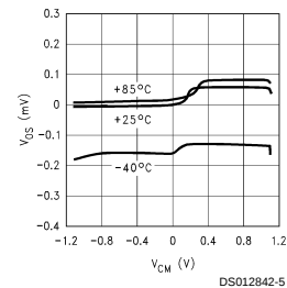
V_{OS} vs V_{CM} V_S = \pm 1.1\text{V}
