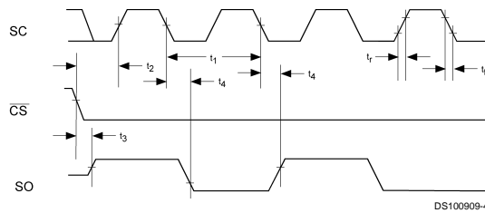
FIGURE 2. Data Output Timing Diagram
