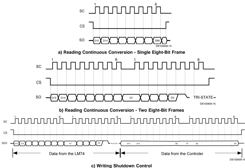
FIGURE 7. Timing Diagrams
