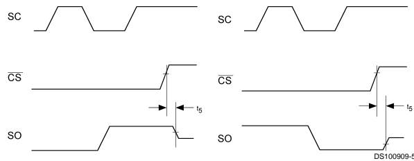
FIGURE 3. TRI-STATE Data Output Timing Diagram
