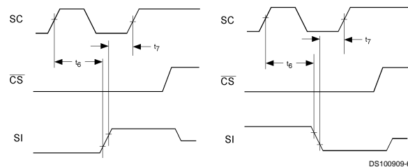
FIGURE 4. Data Input Timing Diagram
