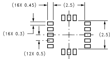
RECOMMENDED LAND PATTERN 1:1 RATIO WITH PACKAGE SOLDER PADS
