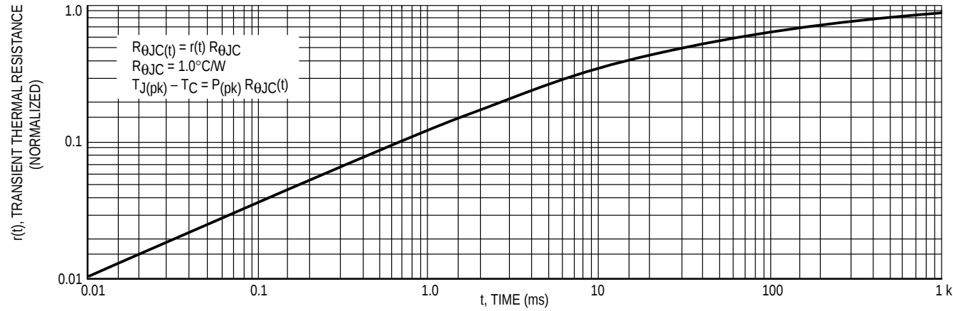
Figure 17. Thermal Response
