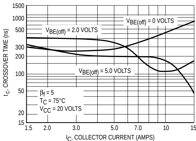
Figure 11. Crossover Time
