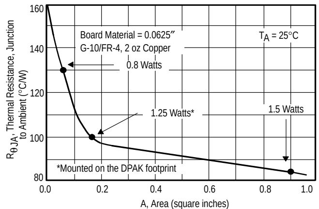
Figure 8. Thermal Resistance versus Collector Pad Area for the SOT-223 Package (Typical)
