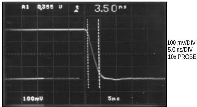
Figure 9. Fall Time for MC13281B
