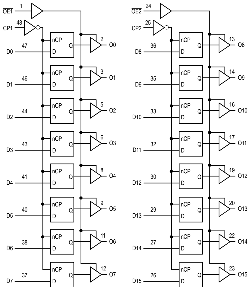
Figure 2. Logic Diagram
