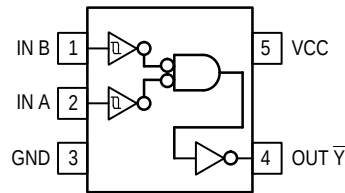
Figure 1. 5-Lead SOT-353 Pinout (Top View)
