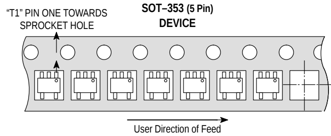
Figure 9. Reel Configuration
