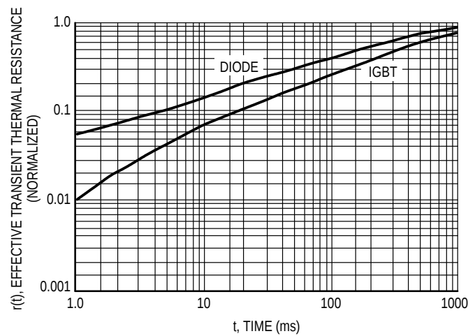
Figure 17. Thermal Response
