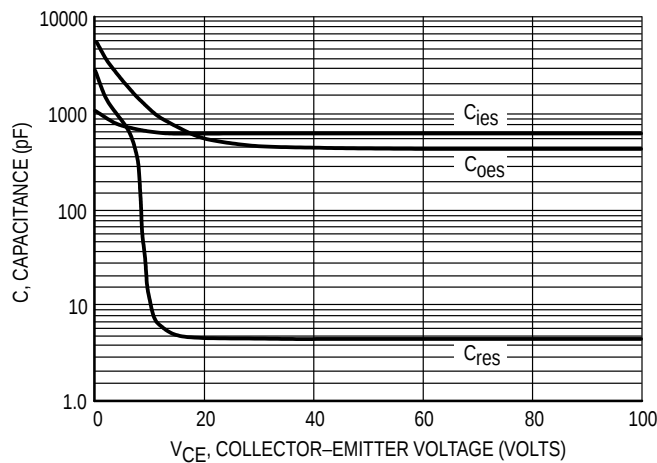
Figure 15. Capacitance Variation
