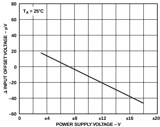
TPC 2. Input Offset Voltage vs. Power Supply Voltage
