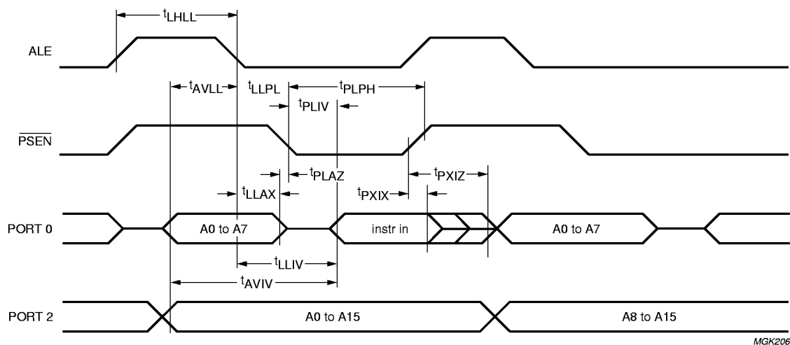
Fig.33 External program memory read cycle.
