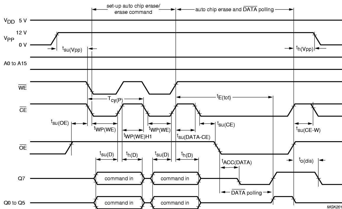
Fig.24 Automatic chip erase timing waveform.
