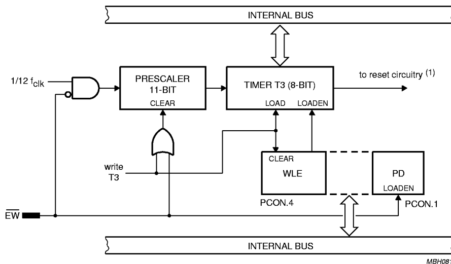
Fig.14 Watchdog Timer block diagram.
