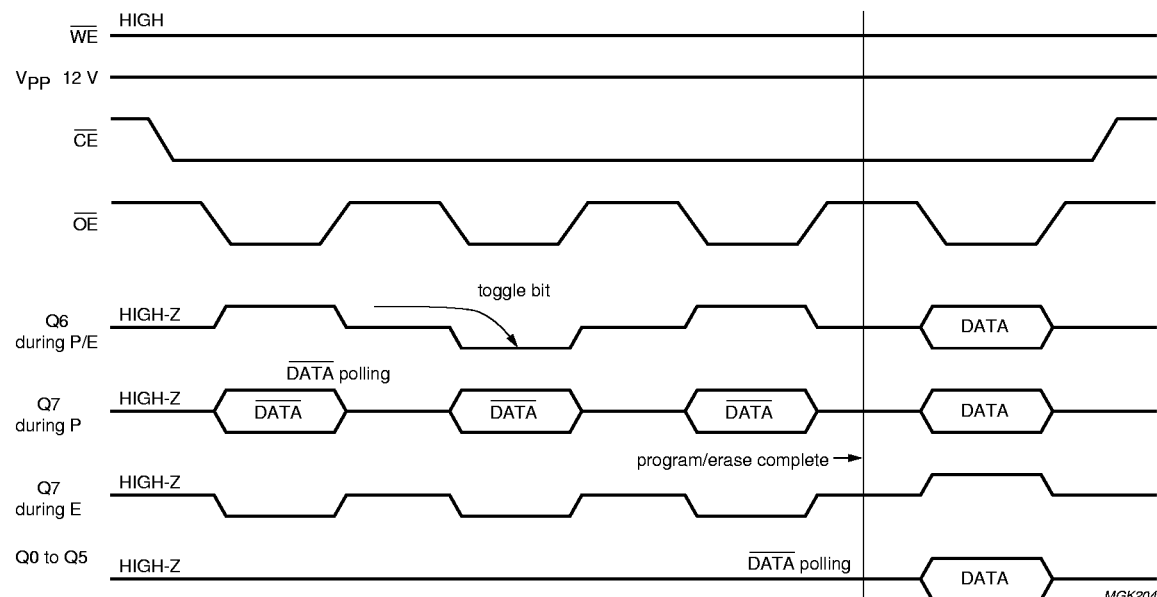
Fig.27 Toggle bit, \overline{DATA} polling timing waveform.
