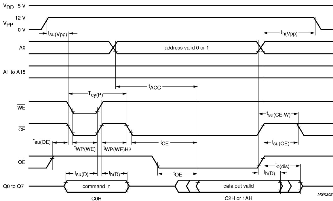
Fig.26 V_{PP} = V_{PPH} (high voltage) identification code read timing waveform.
