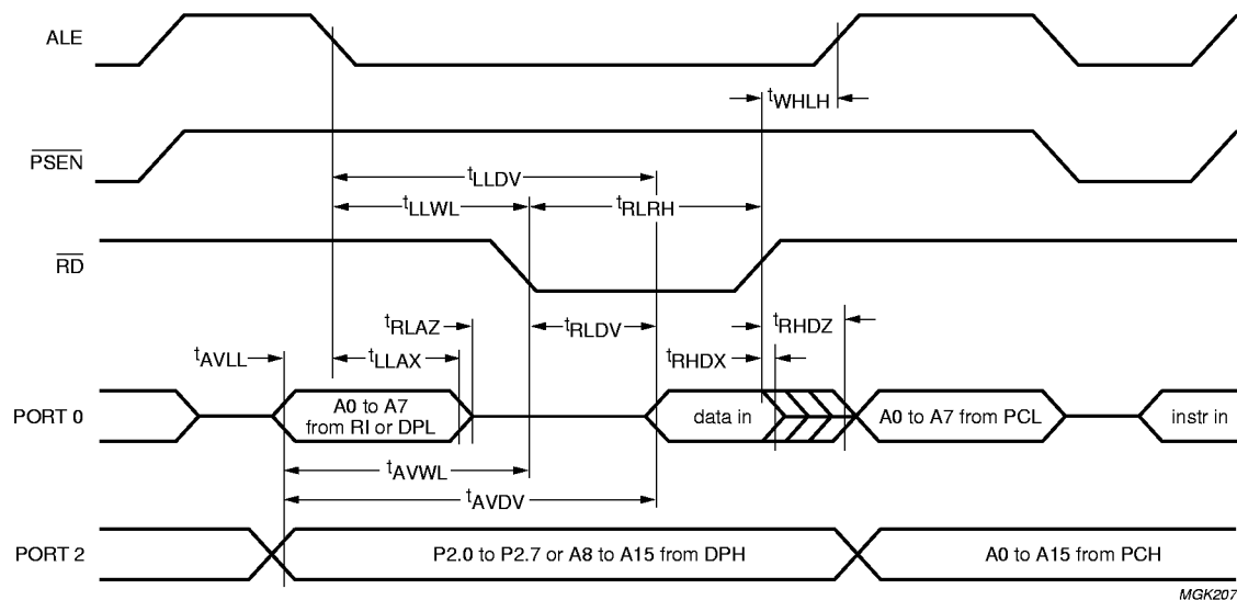
Fig.34 External data memory read cycle.
