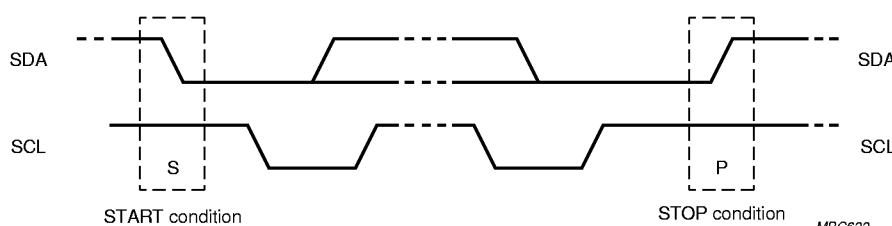
Fig 7. START and STOP conditions on the I 2 C-bus.
