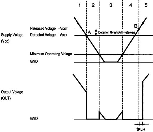
FIG. 2 Operation Diagram
