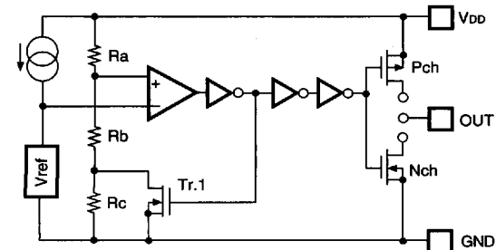
FIG. 1 Block Diagram
