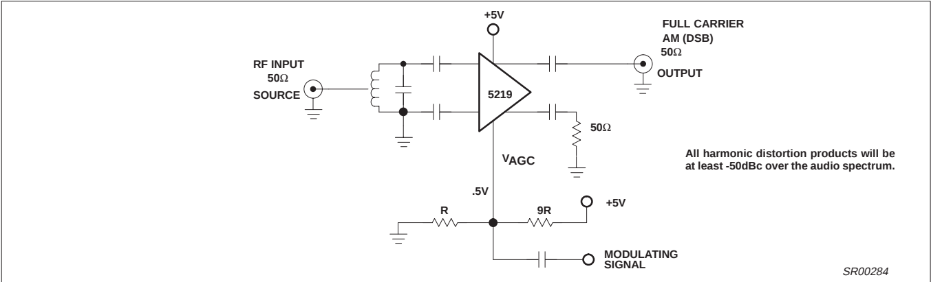
Figure 12. AM Modulator
