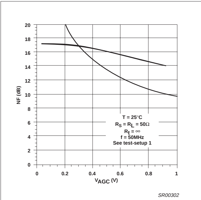
Figure 30. Noise Figure vs V_{AGC}
