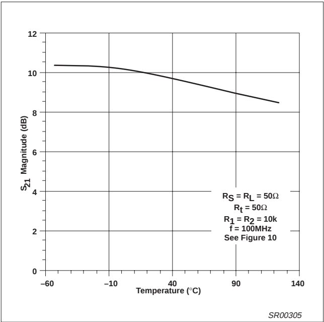
Figure 33. Fixed Gain vs Temperature
