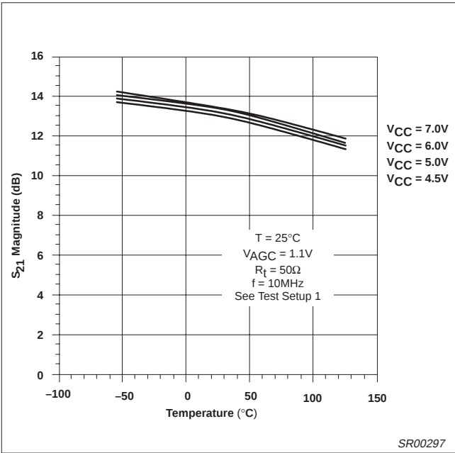
Figure 25. Insertion Gain vs Temperature and V_{CC}
