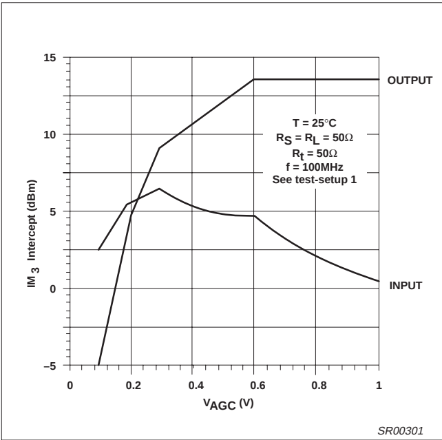
Figure 29. Third-Order Intermodulation Intercept vs V_{AGC}
