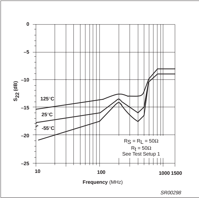
Figure 26. Output Return Loss vs Frequency
