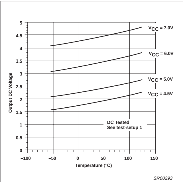
Figure 21. Output Bias Voltage vs Temperature and V_{CC}
