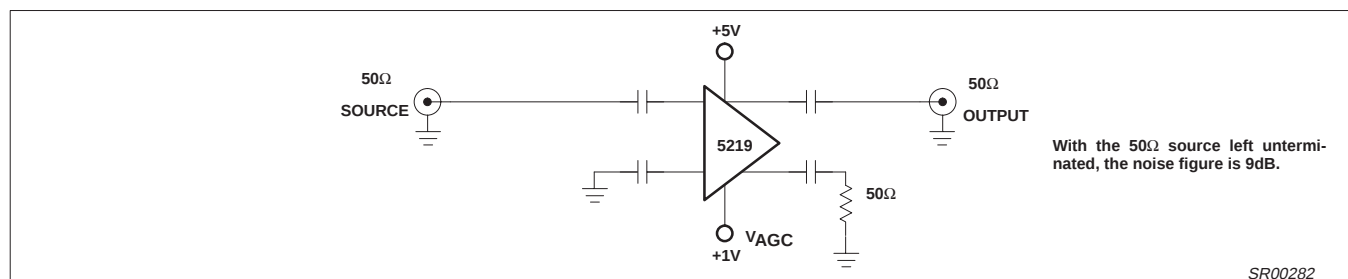
Figure 10. Underterminated Configuration
