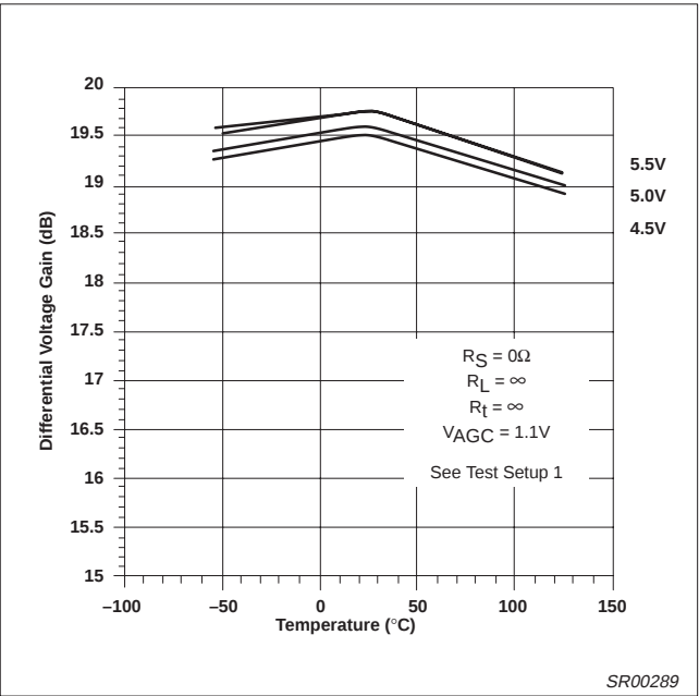
Figure 17. Voltage Gain vs Temperature and V_{CC}
