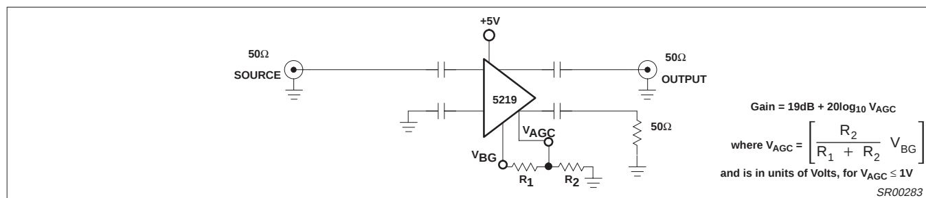
Figure 11. User-Programmable Fixed Gain Block
