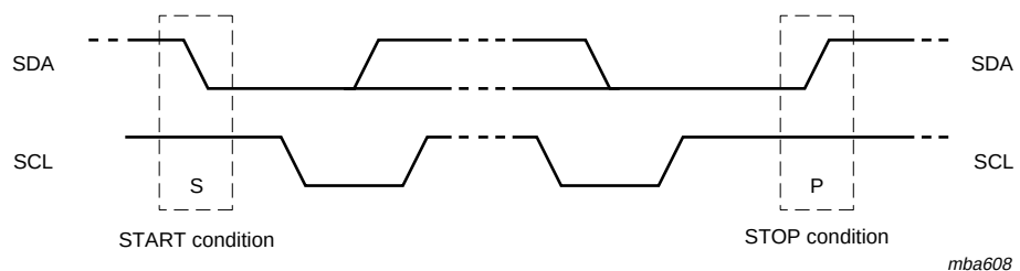
Fig 13. START and STOP conditions
