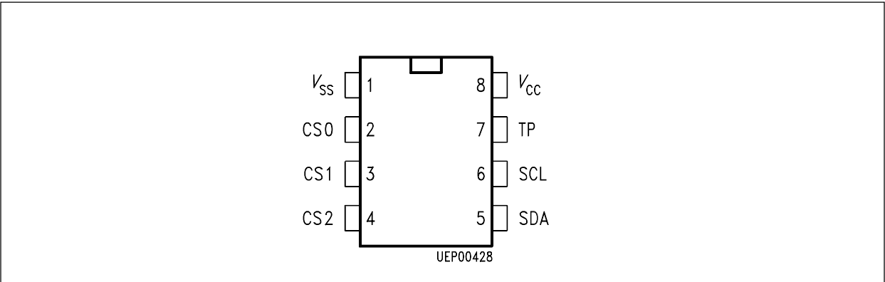
Pin Configuration (top view)
