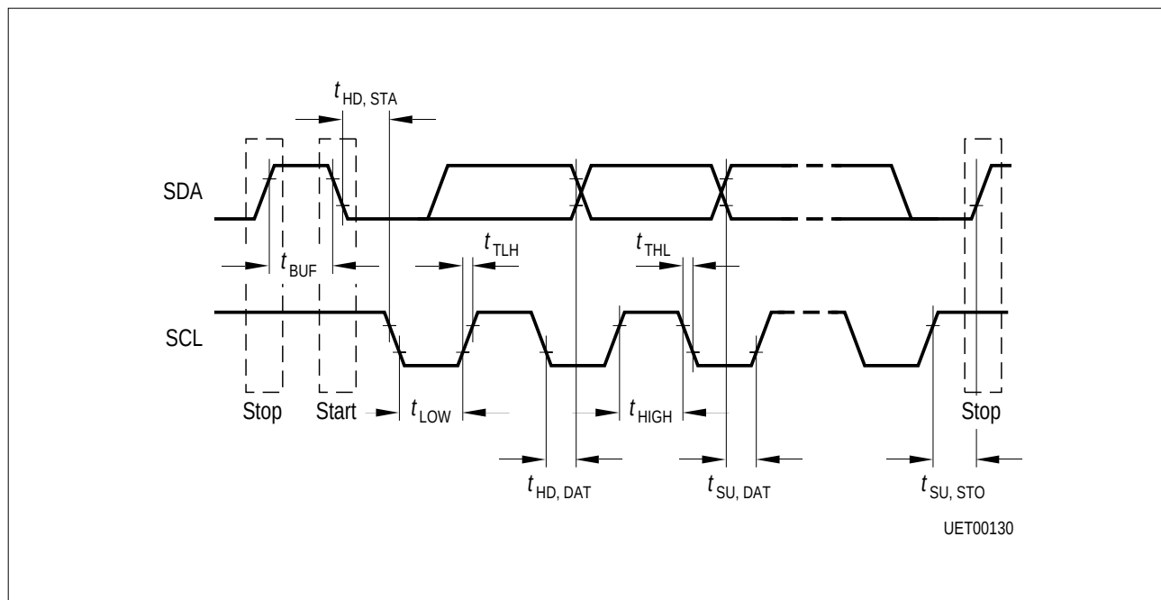
Figure 3 I²C-Bus Timing
