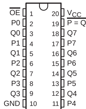
SN54F520 . . . J PACKAGE SN74F520 . . . DW OR N PACKAGE (TOP VIEW)
